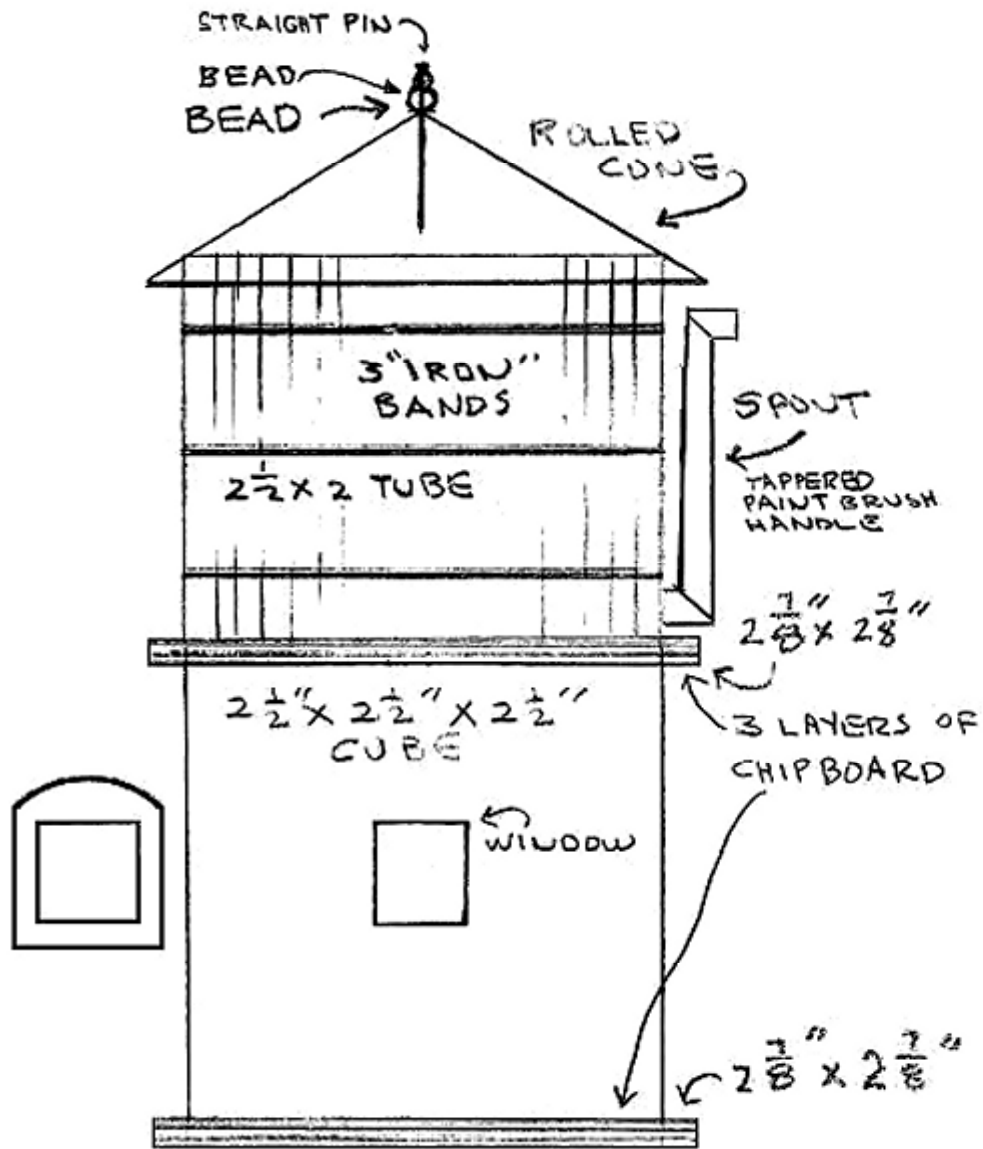
water tank - side
